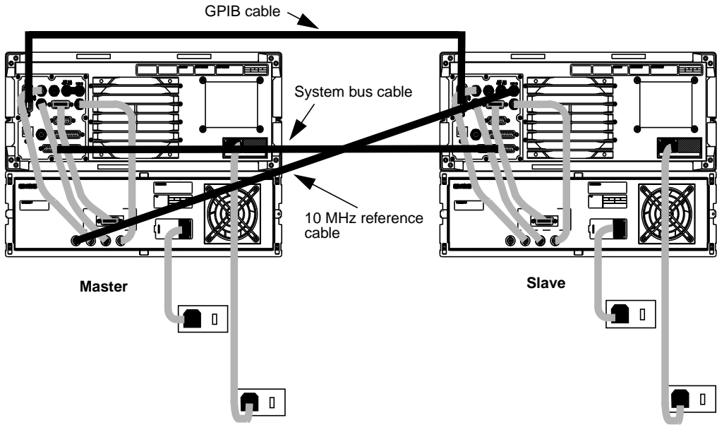
Figure 2-2 Rear panel connections
