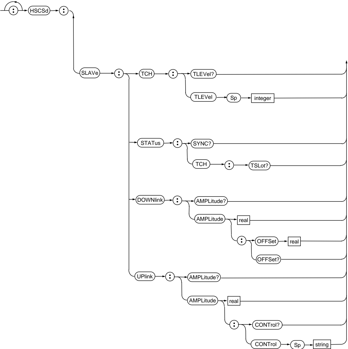
Figure 5-4 HSCSD command syntax (slave unit)
